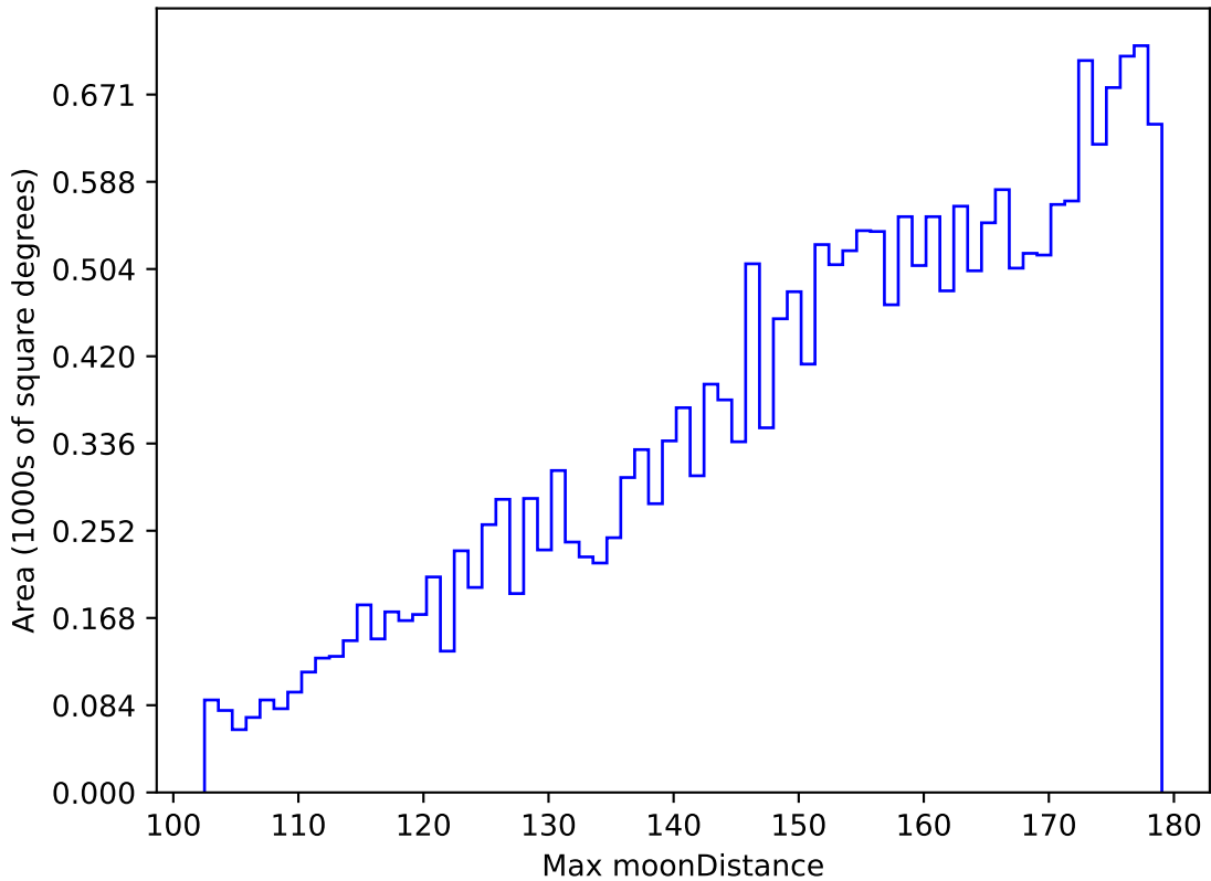
too_elab_r256_d2_gz_v3.4_10yrs All sky u band: Max moonDistance
