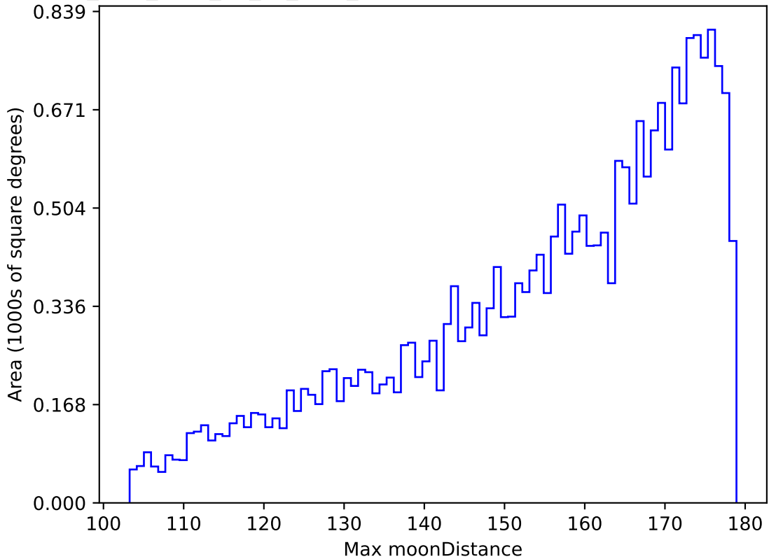
too_elab_r256_d2_gz_v3.4_10yrs All sky g band: Max moonDistance
