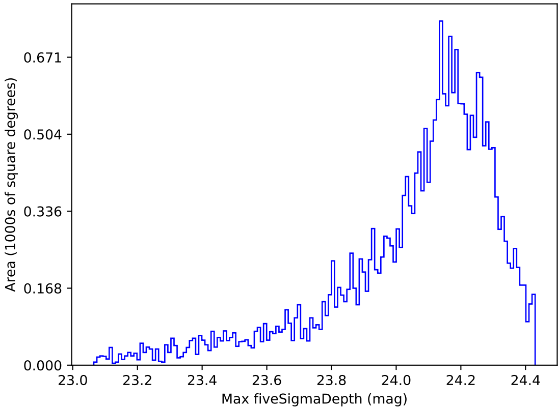
too_elab_r256_d2_gz_v3.4_10yrs Yr 1 i band: Max fiveSigmaDepth
