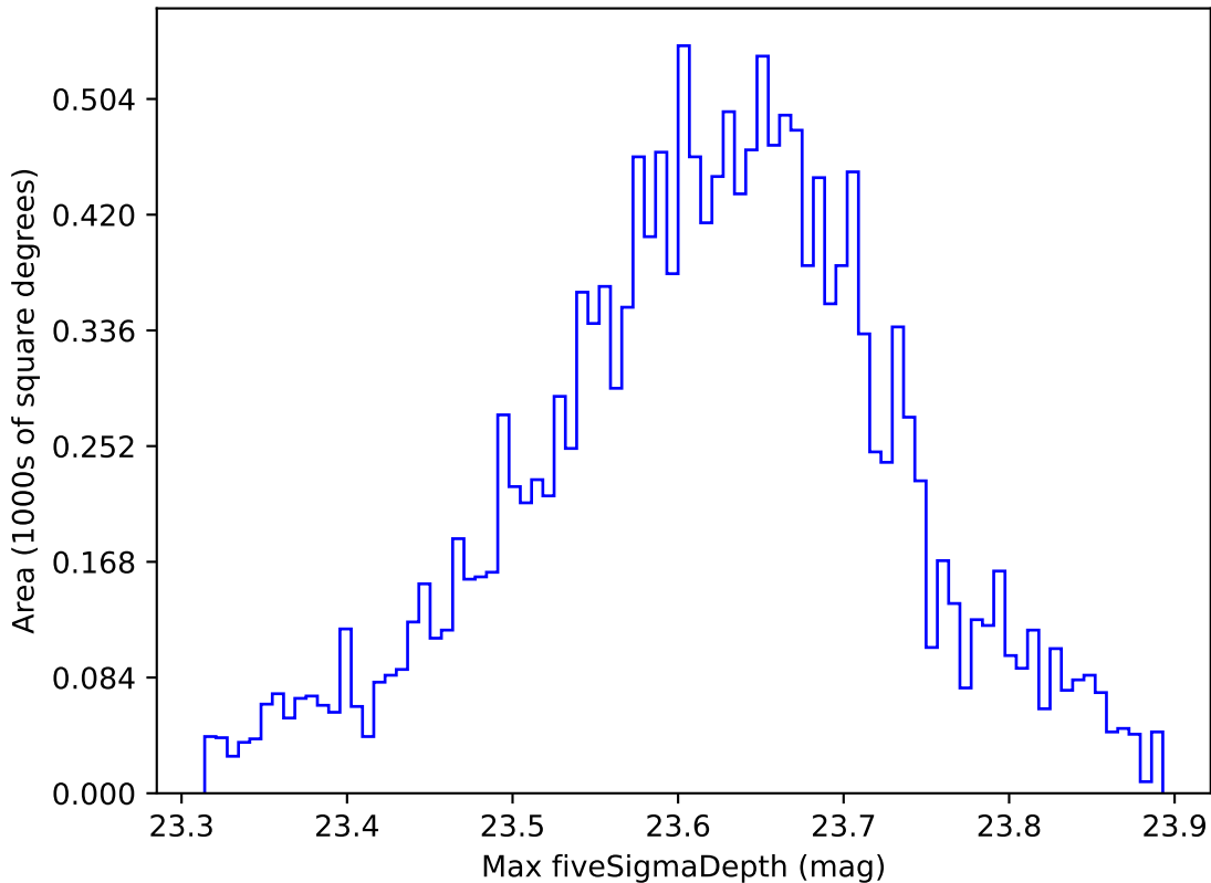
too_elab_r256_d2_gz_v3.4_10yrs WFD z band: Max fiveSigmaDepth
