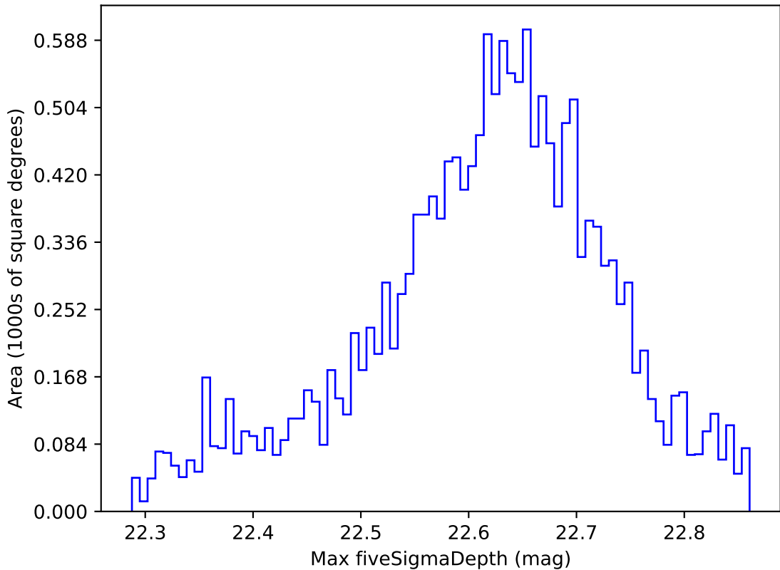
too_elab_r256_d2_gz_v3.4_10yrs WFD y band: Max fiveSigmaDepth
