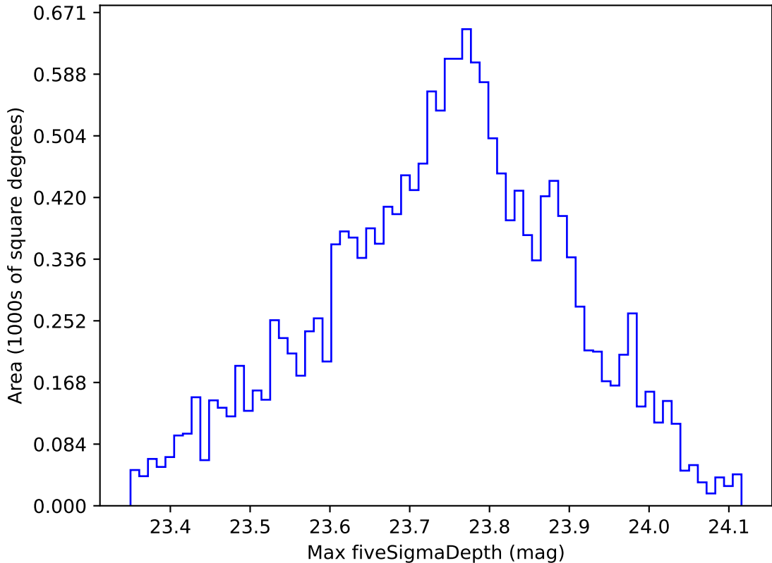
too_elab_r256_d2_gz_v3.4_10yrs WFD u band: Max fiveSigmaDepth
