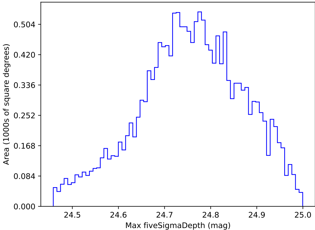
too_elab_r256_d2_gz_v3.4_10yrs WFD r band: Max fiveSigmaDepth
