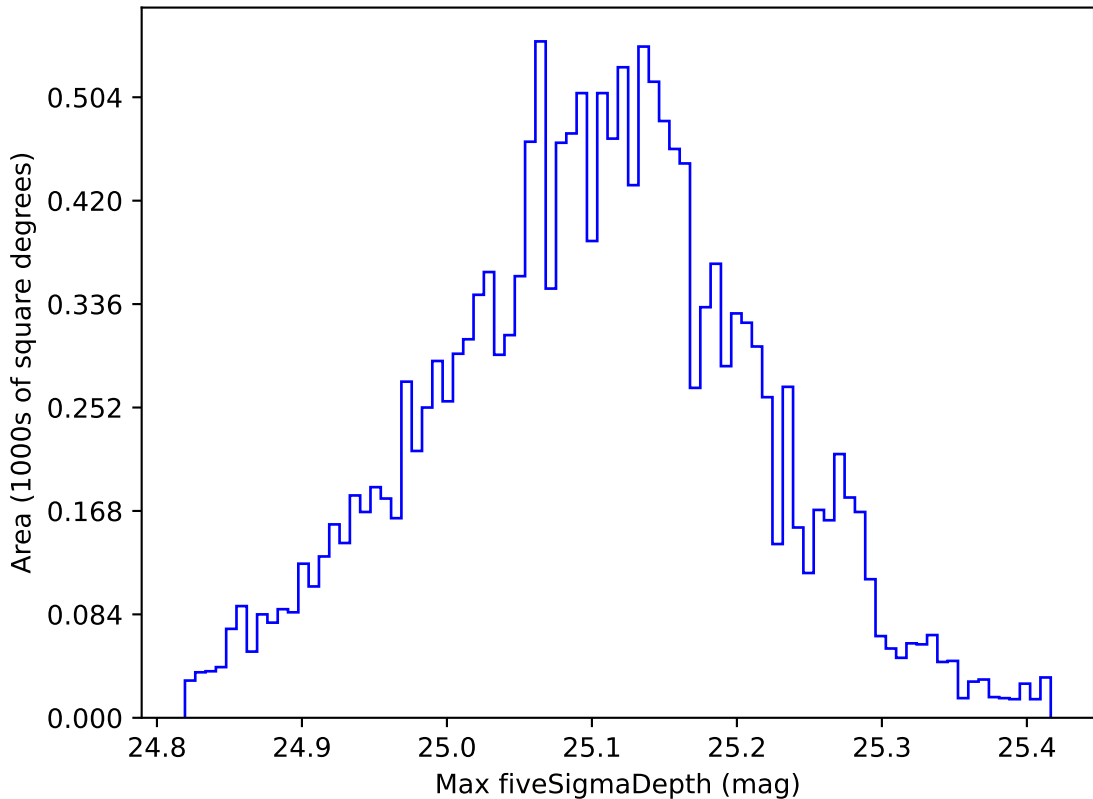
too_elab_r256_d2_gz_v3.4_10yrs WFD g band: Max fiveSigmaDepth
