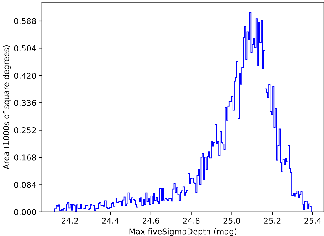
too_elab_r256_d2_gz_v3.4_10yrs All sky g band: Max fiveSigmaDepth
