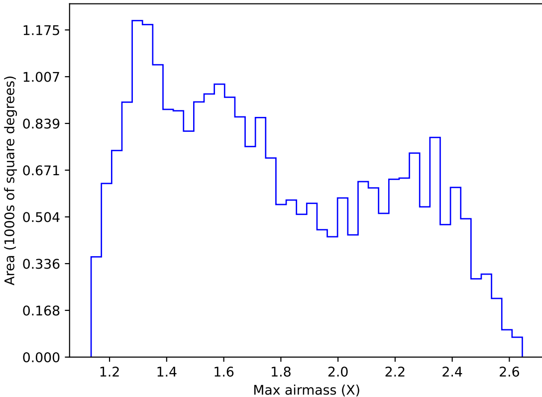
too_elab_r256_d2_gz_v3.4_10yrs Yr 1 r band: Max airmass
