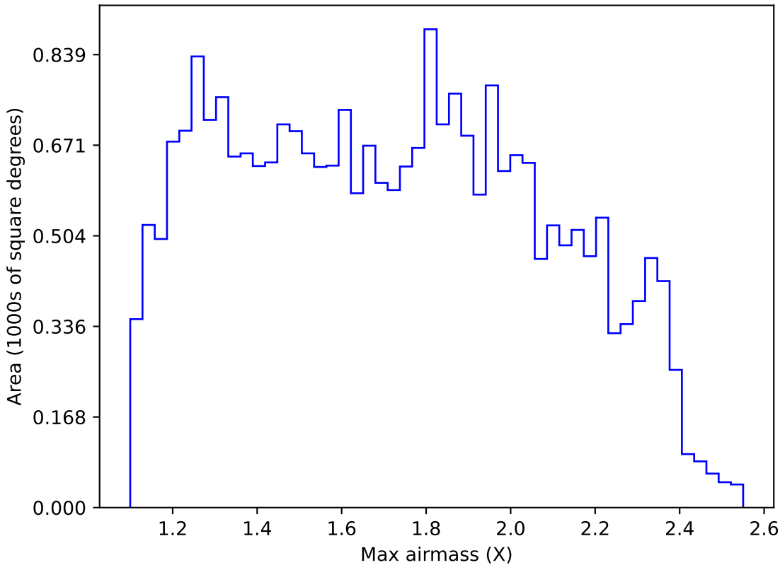
too_elab_r256_d2_gz_v3.4_10yrs Yr 1 g band: Max airmass
