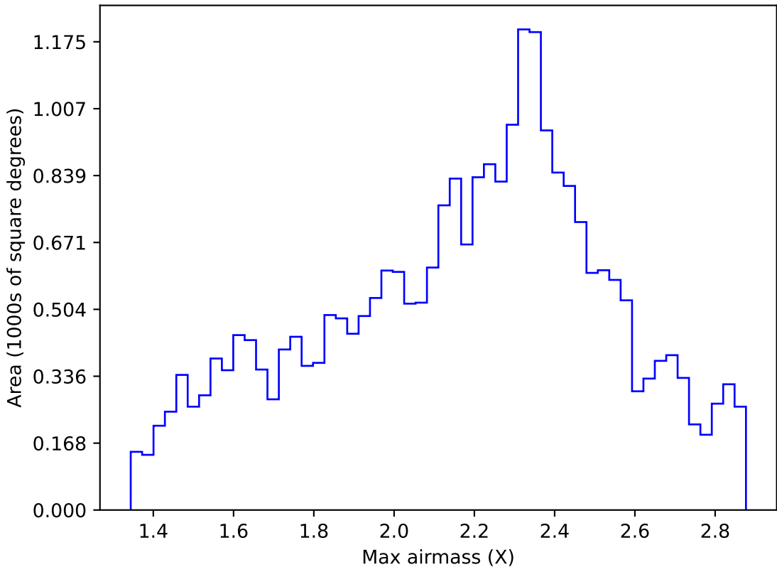
too_elab_r256_d2_gz_v3.4_10yrs Yr 1 all bands: Max airmass
