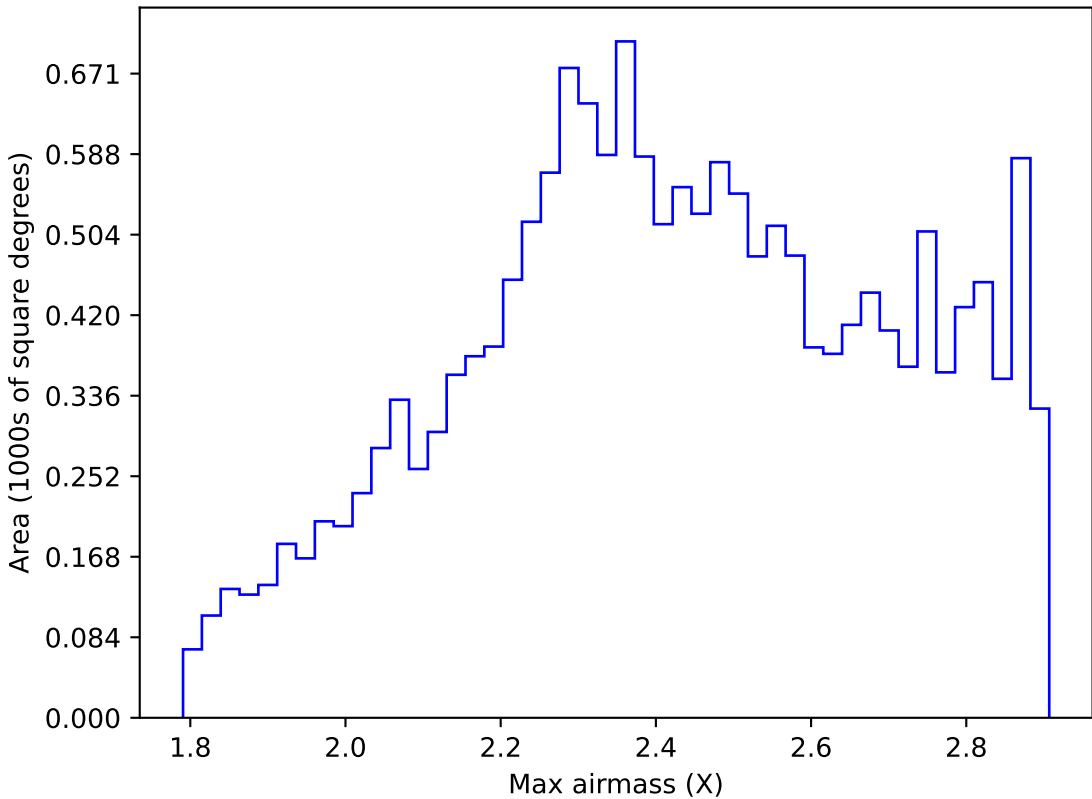
too_elab_r256_d2_gz_v3.4_10yrs WFD z band: Max airmass
