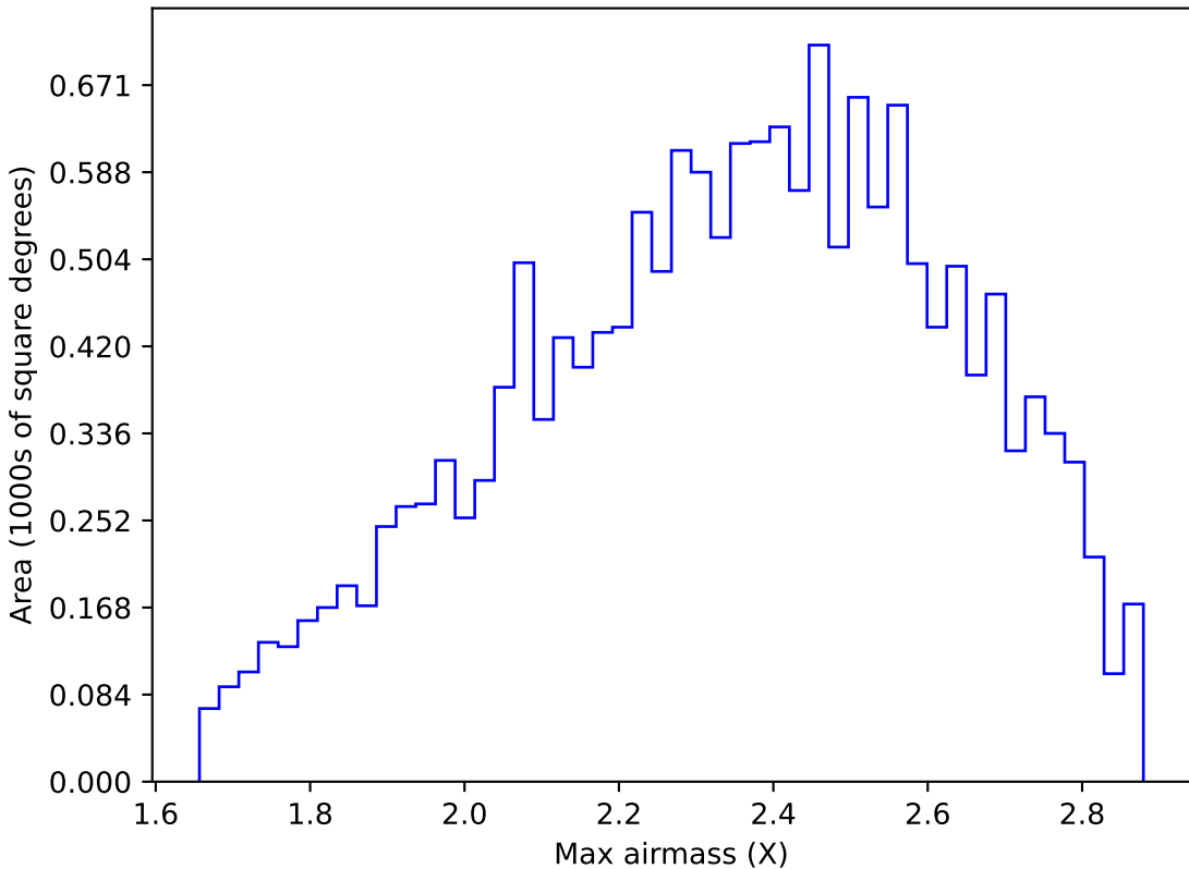
too_elab_r256_d2_gz_v3.4_10yrs WFD y band: Max airmass
