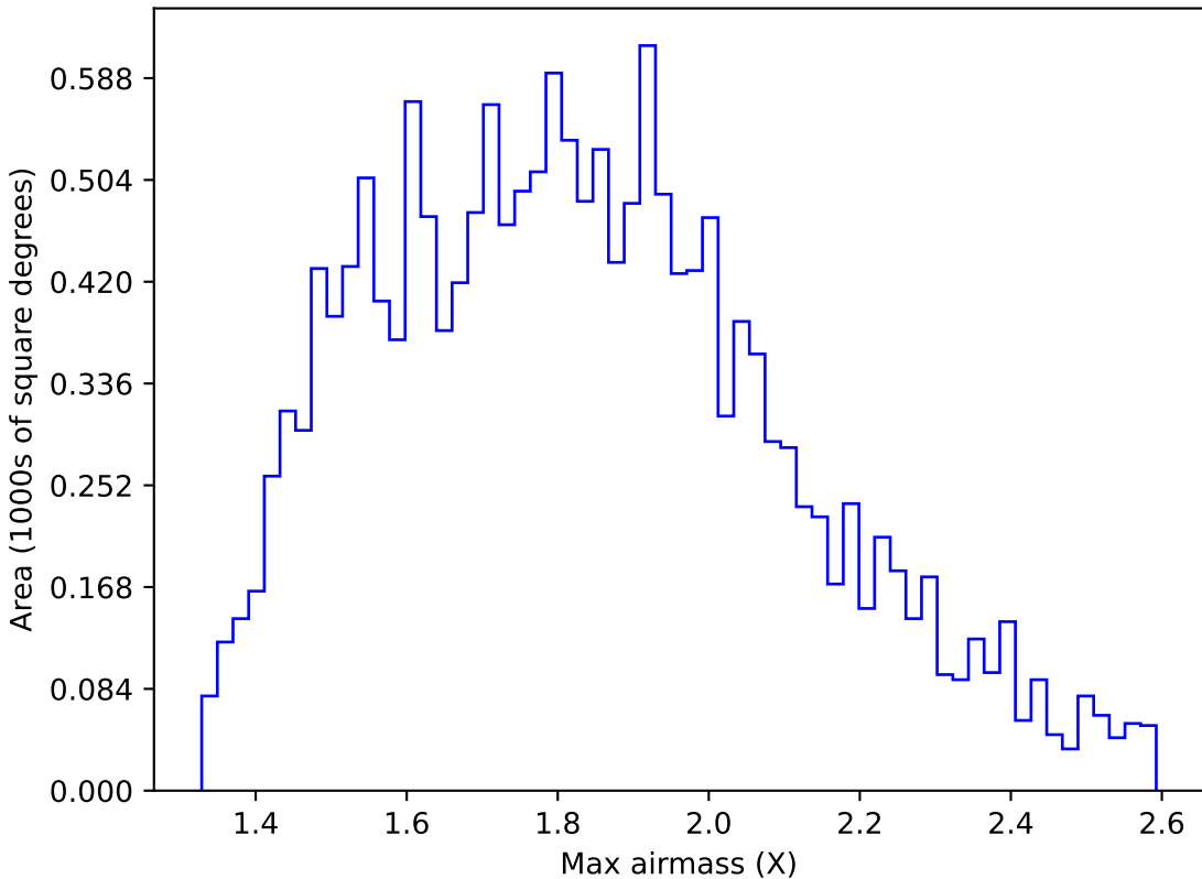
too_elab_r256_d2_gz_v3.4_10yrs WFD u band: Max airmass
