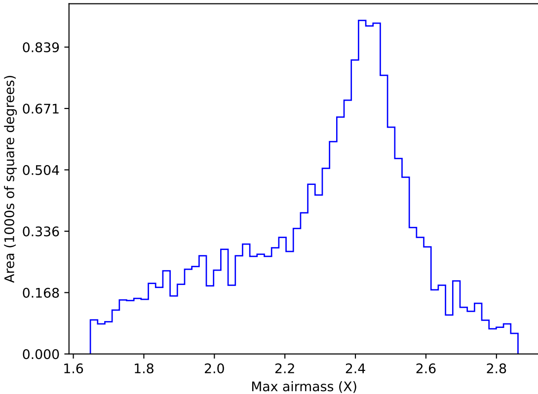
too_elab_r256_d2_gz_v3.4_10yrs WFD r band: Max airmass
