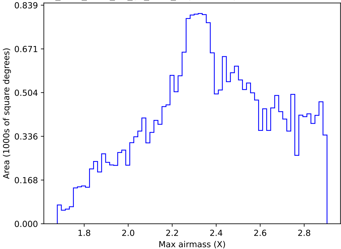
too_elab_r256_d2_gz_v3.4_10yrs All sky z band: Max airmass
