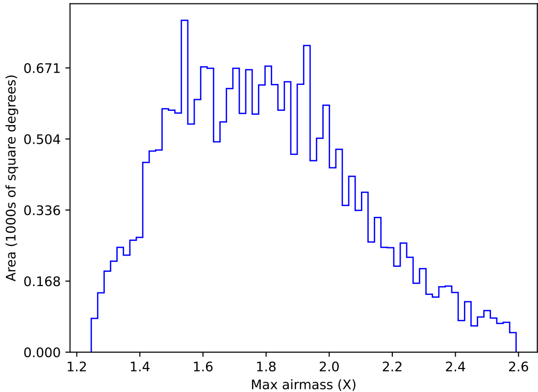
too_elab_r256_d2_gz_v3.4_10yrs All sky u band: Max airmass
