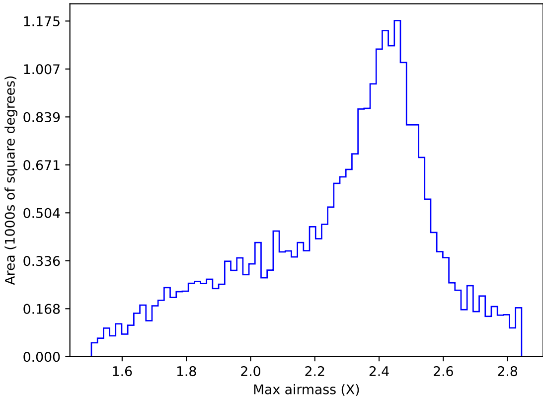
too_elab_r256_d2_gz_v3.4_10yrs All sky r band: Max airmass
