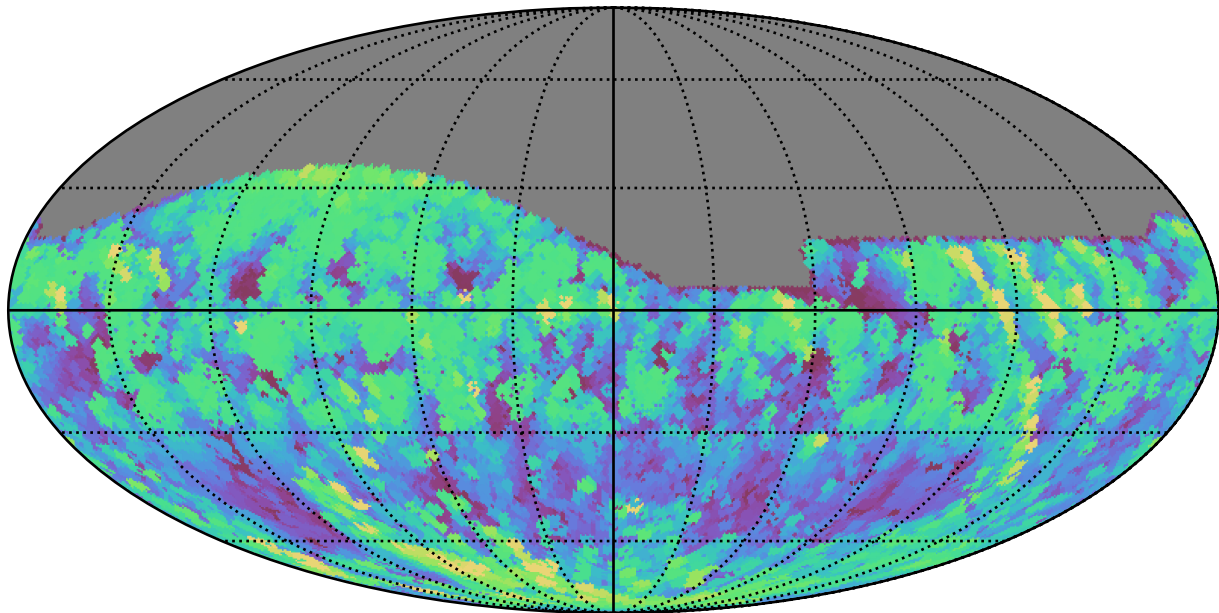
too_elab_r256_d2_gz_v3.4_10yrs All sky g band: Max airmass
