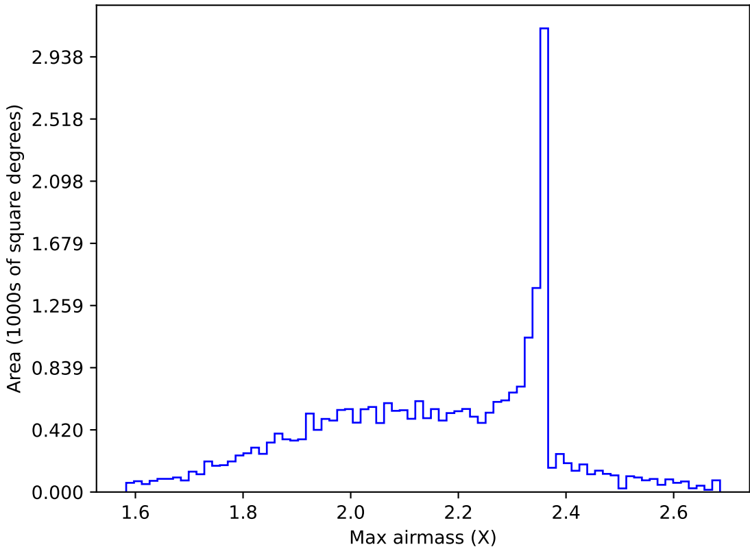
too_elab_r256_d2_gz_v3.4_10yrs All sky g band: Max airmass
