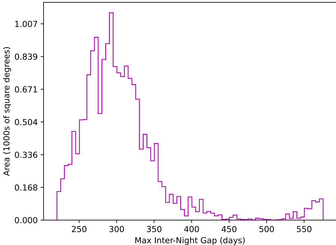
too_elab_r256_d2_gz_v3.4_10yrs WFD z band: Max Inter-Night Gap
