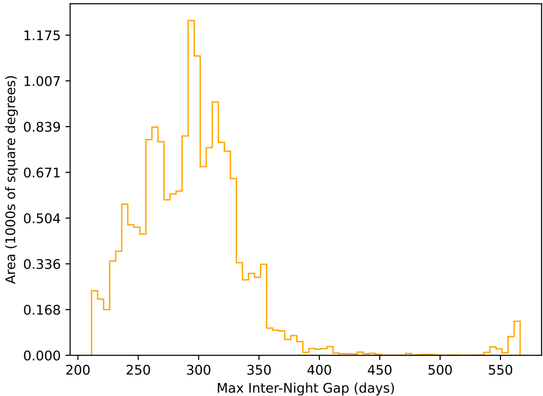
too_elab_r256_d2_gz_v3.4_10yrs WFD r band: Max Inter-Night Gap
