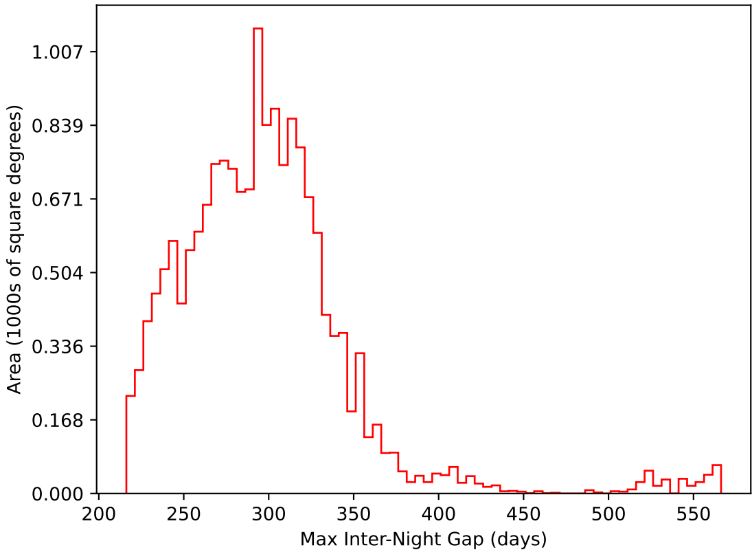
too_elab_r256_d2_gz_v3.4_10yrs WFD i band: Max Inter-Night Gap
