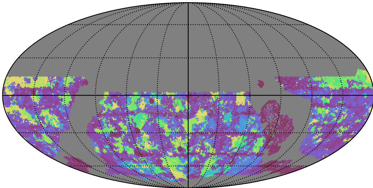
too_elab_r256_d2_gz_v3.4_10yrs WFD g band: Max Inter-Night Gap
