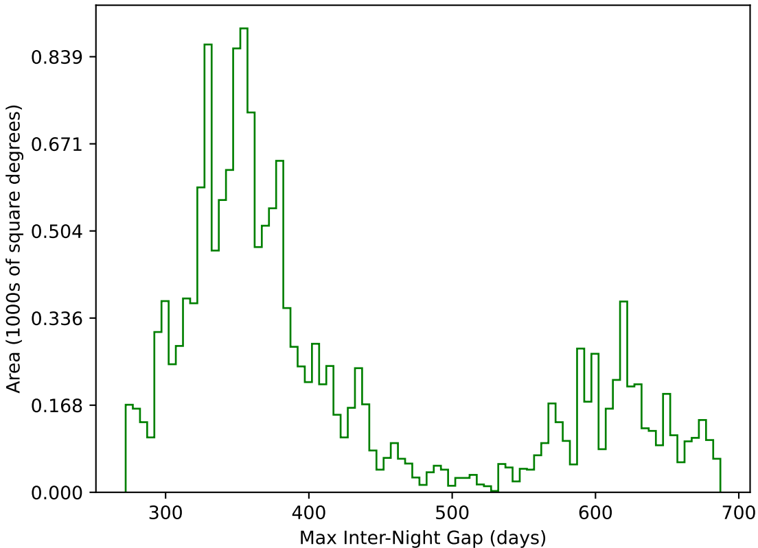
too_elab_r256_d2_gz_v3.4_10yrs WFD g band: Max Inter-Night Gap
