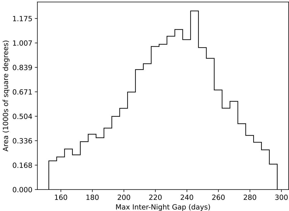
too_elab_r256_d2_gz_v3.4_10yrs WFD all bands: Max Inter-Night Gap
