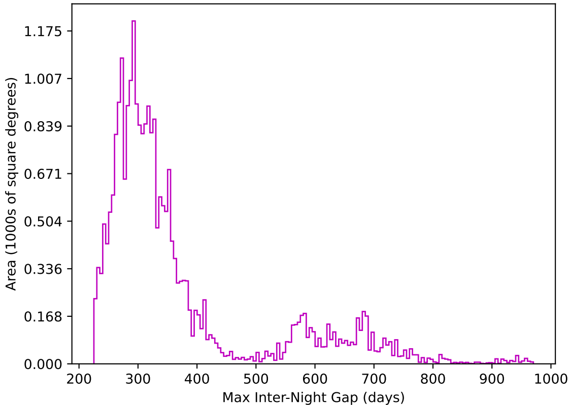
too_elab_r256_d2_gz_v3.4_10yrs All sky z band: Max Inter-Night Gap
