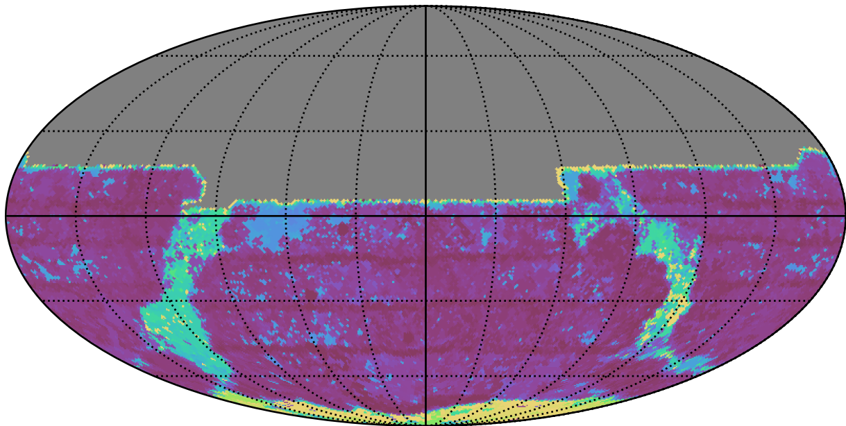
too_elab_r256_d2_gz_v3.4_10yrs All sky y band: Max Inter-Night Gap
