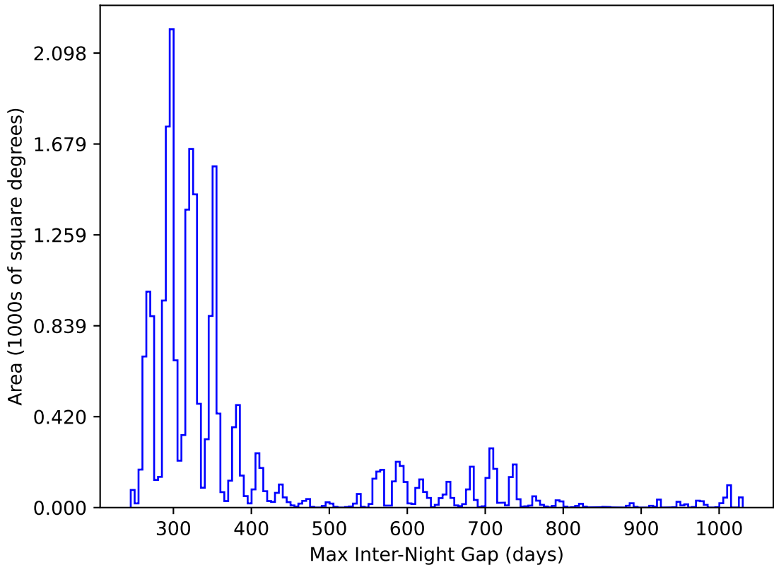
too_elab_r256_d2_gz_v3.4_10yrs All sky y band: Max Inter-Night Gap
