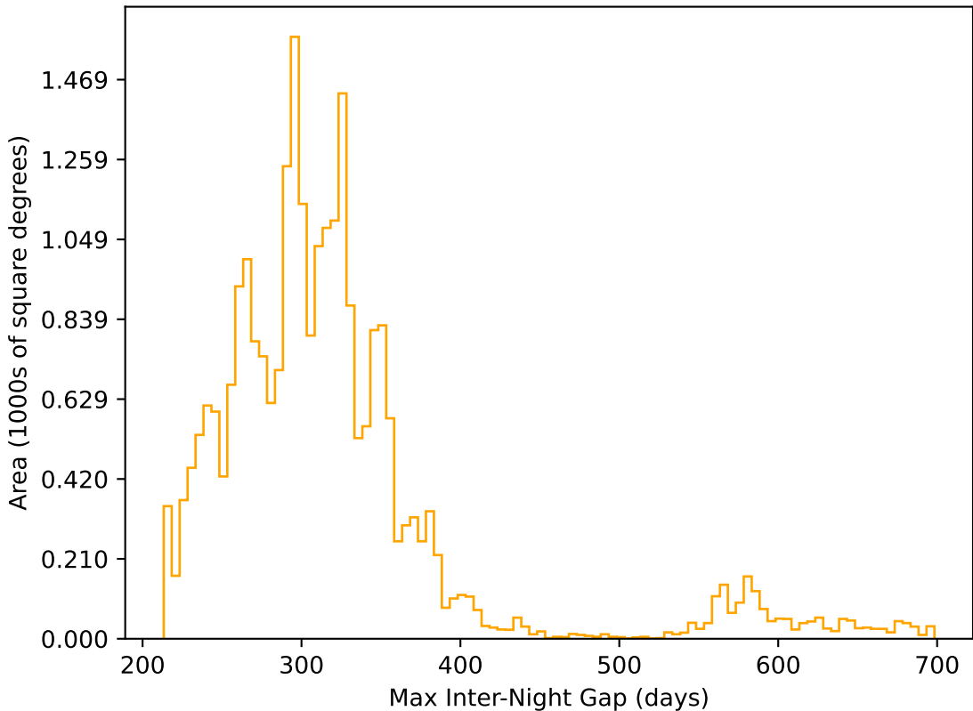
too_elab_r256_d2_gz_v3.4_10yrs All sky r band: Max Inter-Night Gap
