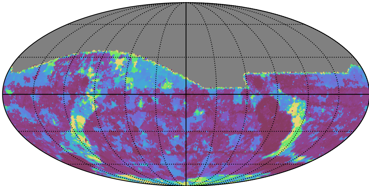
too_elab_r256_d2_gz_v3.4_10yrs All sky g band: Max Inter-Night Gap
