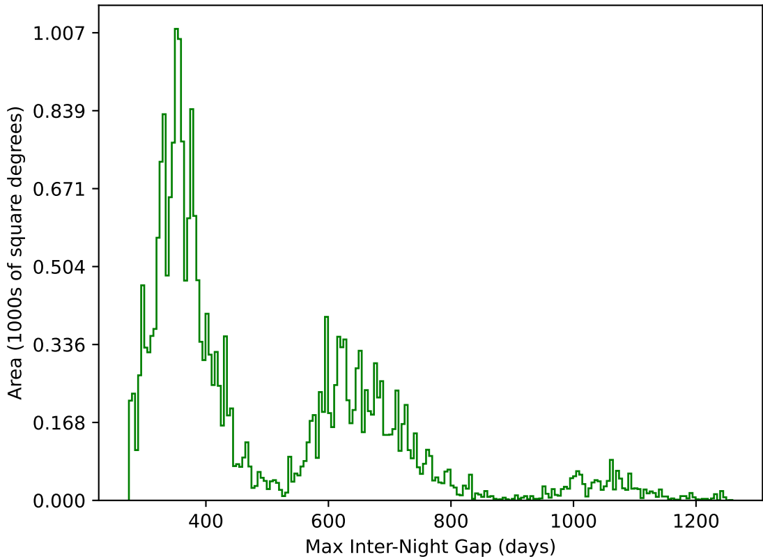
too_elab_r256_d2_gz_v3.4_10yrs All sky g band: Max Inter-Night Gap
