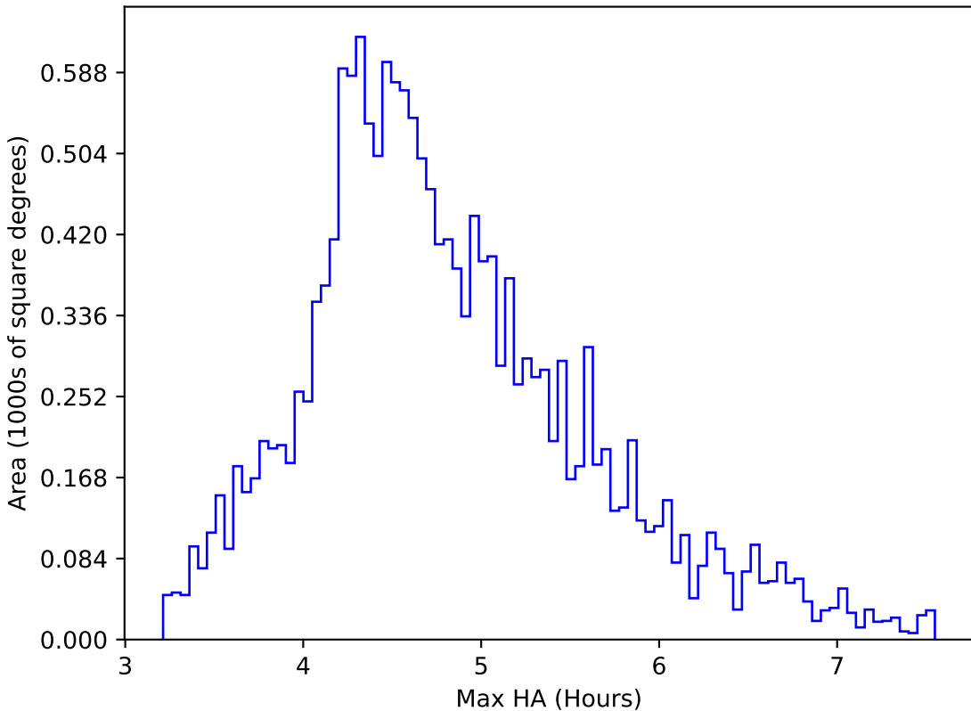
too_elab_r256_d2_gz_v3.4_10yrs WFD y band: Max HA
