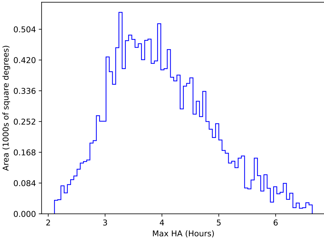
too_elab_r256_d2_gz_v3.4_10yrs WFD u band: Max HA
