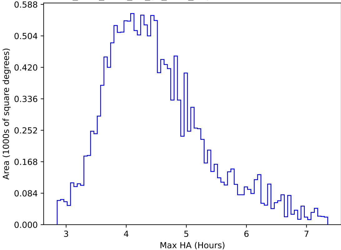
too_elab_r256_d2_gz_v3.4_10yrs WFD r band: Max HA
