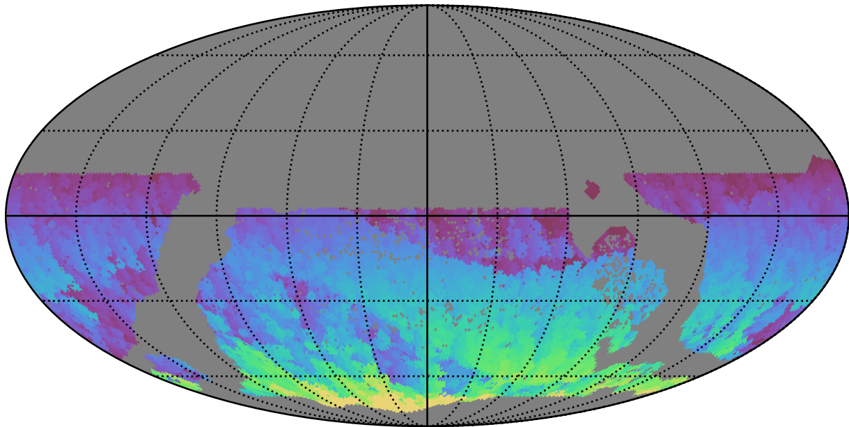
too_elab_r256_d2_gz_v3.4_10yrs WFD i band: Max HA
