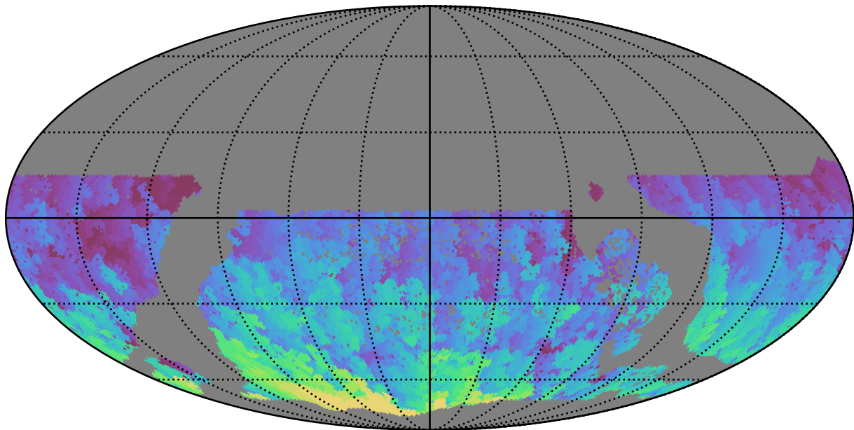
too_elab_r256_d2_gz_v3.4_10yrs WFD g band: Max HA
