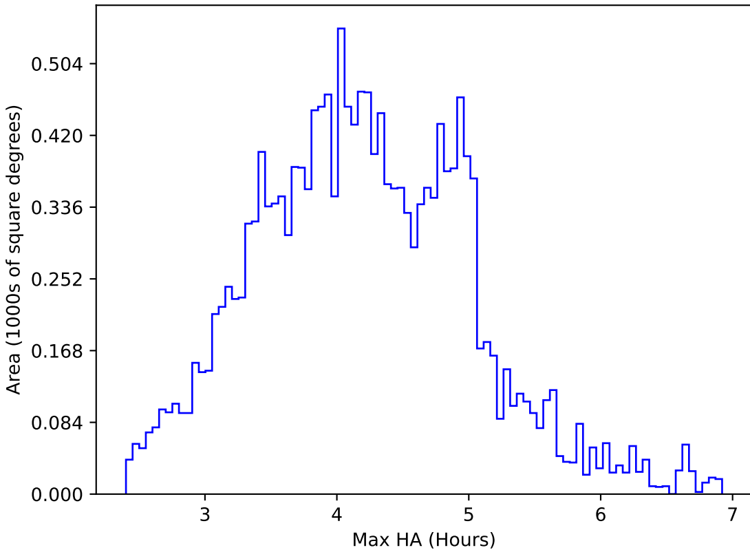
too_elab_r256_d2_gz_v3.4_10yrs WFD g band: Max HA
