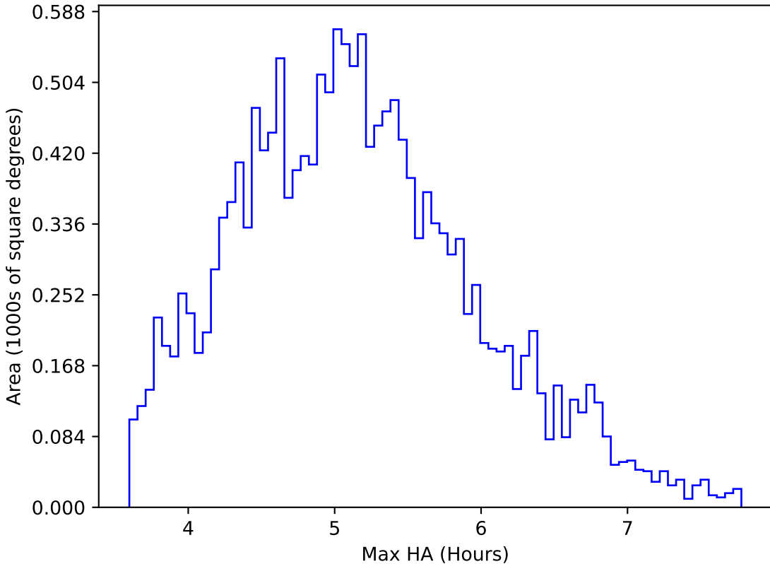
too_elab_r256_d2_gz_v3.4_10yrs WFD all bands: Max HA
