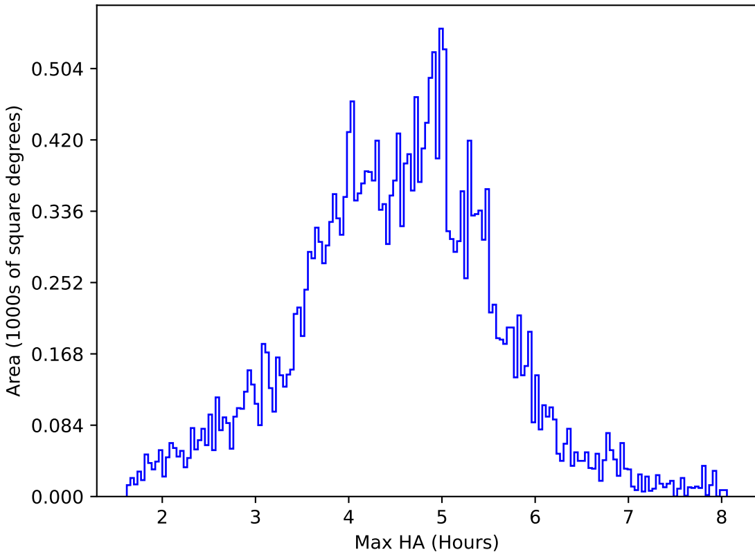
too_elab_r256_d2_gz_v3.4_10yrs All sky z band: Max HA
