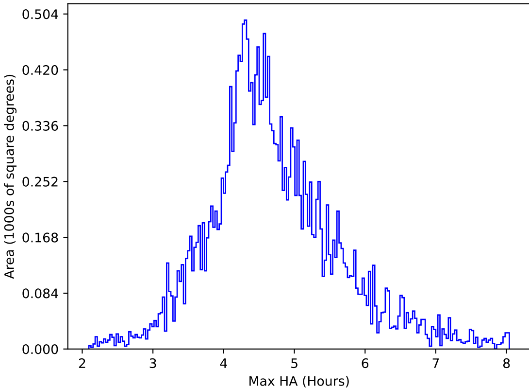
too_elab_r256_d2_gz_v3.4_10yrs All sky y band: Max HA
