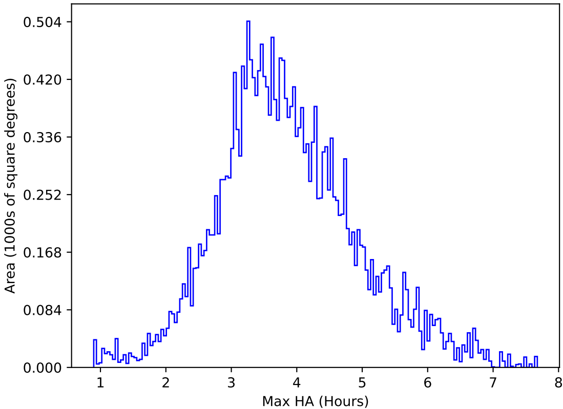
too_elab_r256_d2_gz_v3.4_10yrs All sky u band: Max HA
