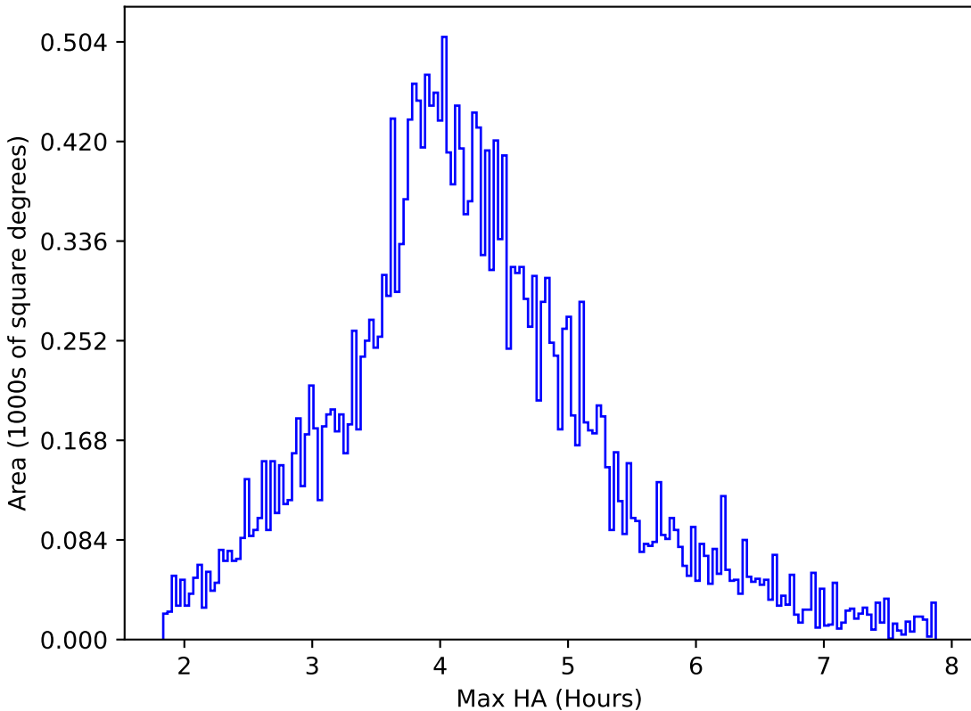
too_elab_r256_d2_gz_v3.4_10yrs All sky r band: Max HA
