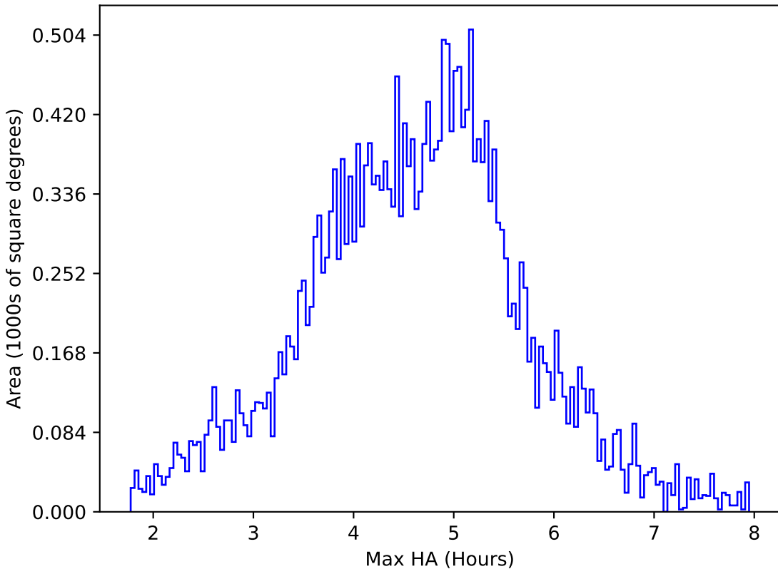
too_elab_r256_d2_gz_v3.4_10yrs All sky i band: Max HA
