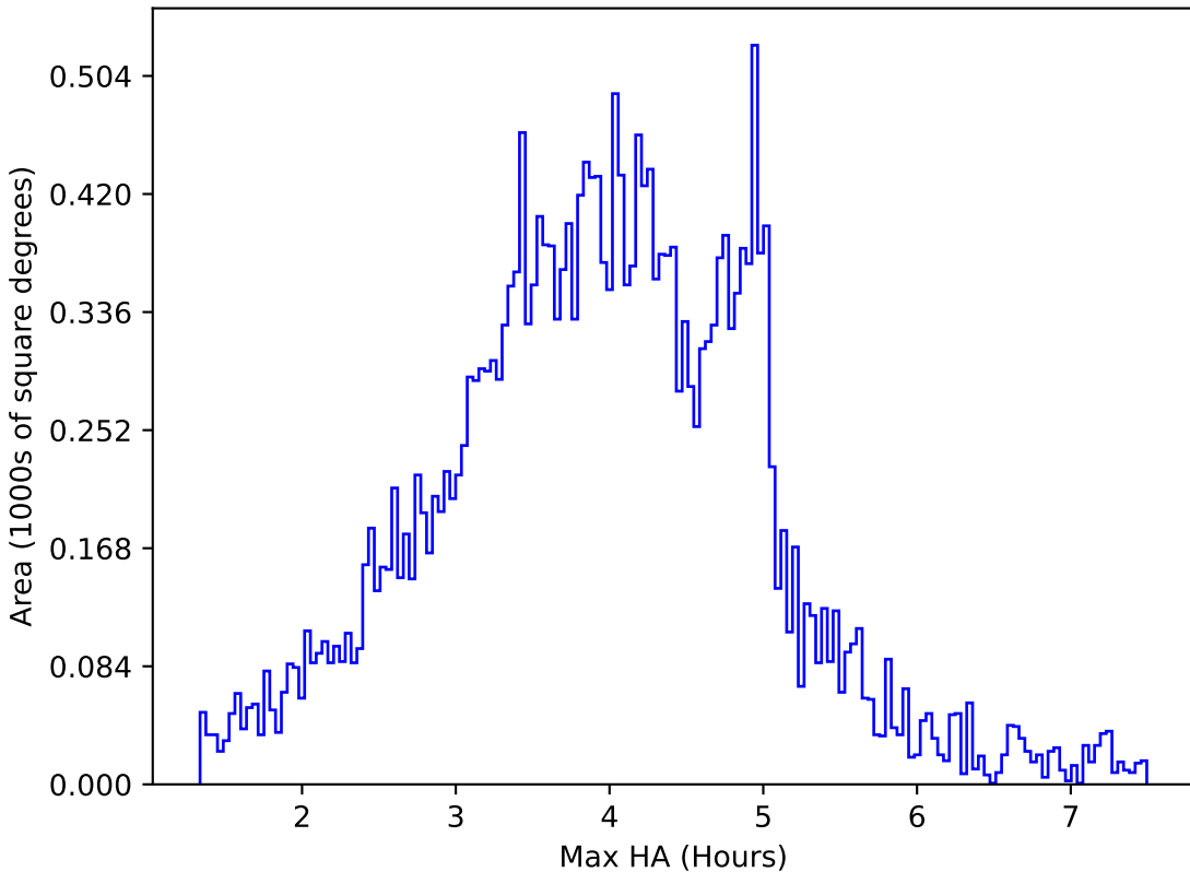
too_elab_r256_d2_gz_v3.4_10yrs All sky g band: Max HA
