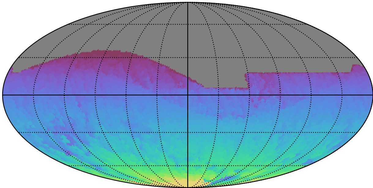
too_elab_r256_d2_gz_v3.4_10yrs All sky all bands: Max HA
