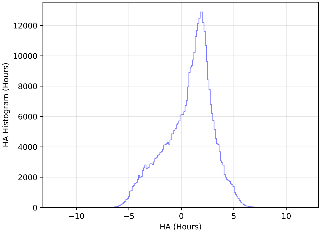
too_elab_r256_d2_gz_v3.4_10yrs WFD z band: HA Histogram
