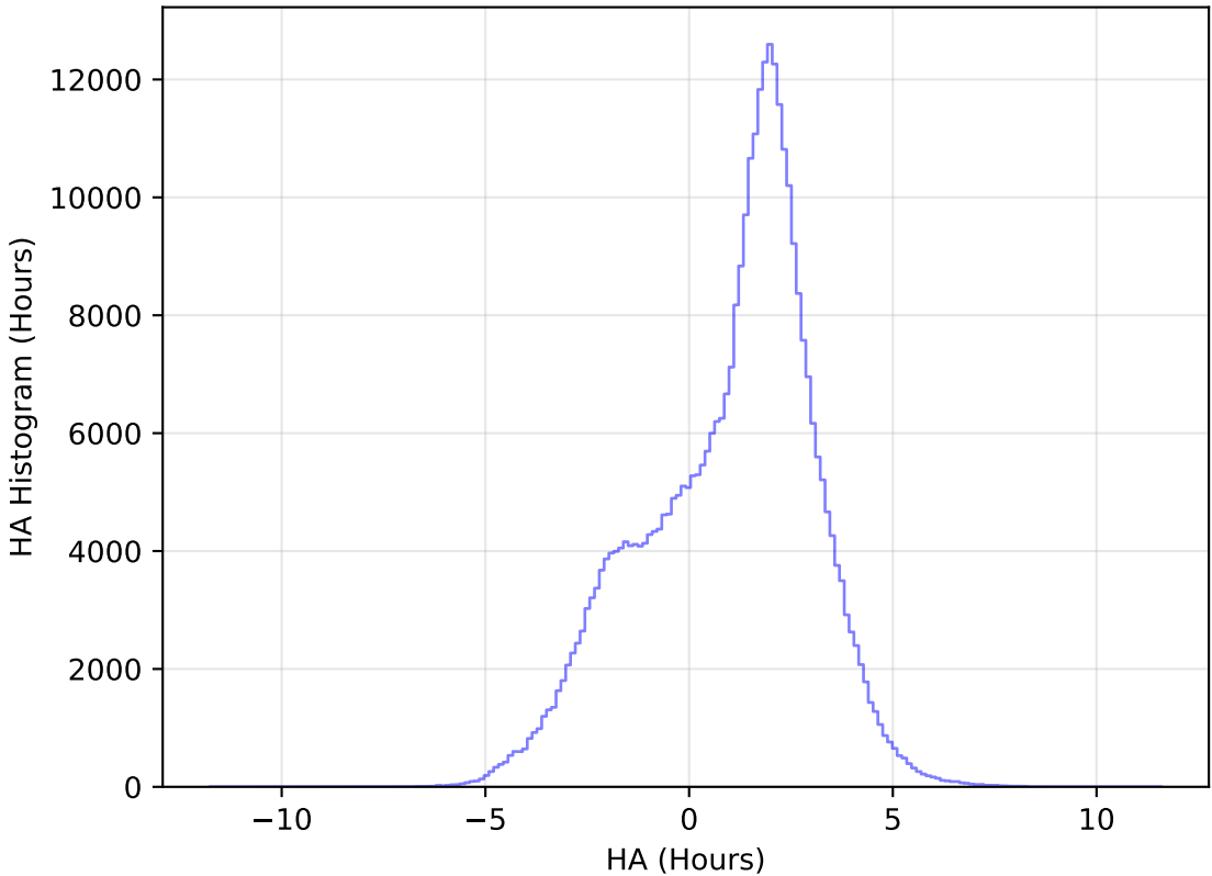
too_elab_r256_d2_gz_v3.4_10yrs WFD y band: HA Histogram
