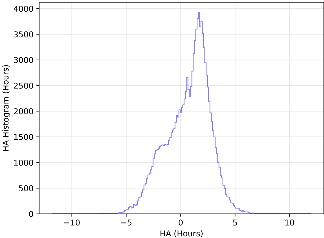
too_elab_r256_d2_gz_v3.4_10yrs WFD u band: HA Histogram
